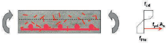
Conventionally reinforced concrete floor study
