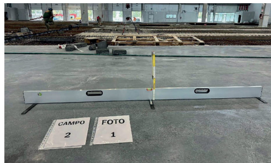
Flatness tests
